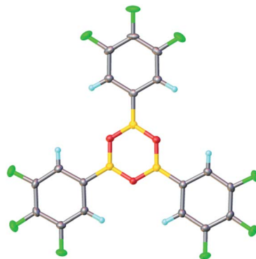
Fig. 4 X-ray structure of 3,4,5-trifluorophenylboroxine 7a in orthorhombic \beta -form at 120 K.
