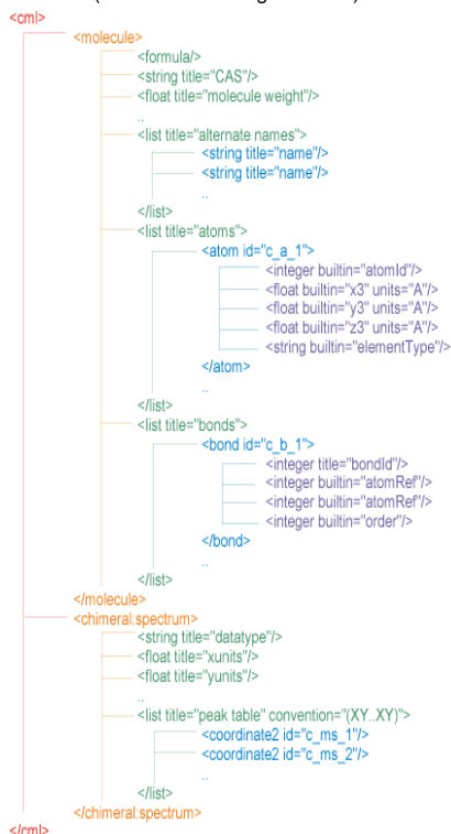
Figure 3: The CML element 'tree'. The molecule contains three lists, one of alternate names, one of atoms with their coordinates and one of bonds and their atom references (the atoms defining the bond)
