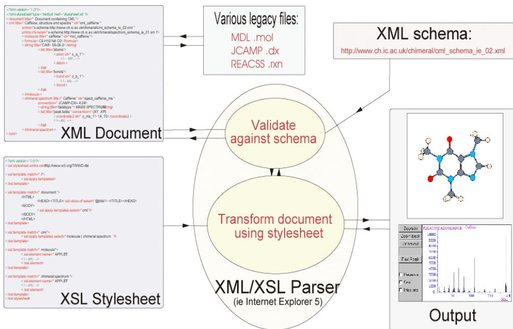
Figure 10: Data flow in an XML/XSL system
