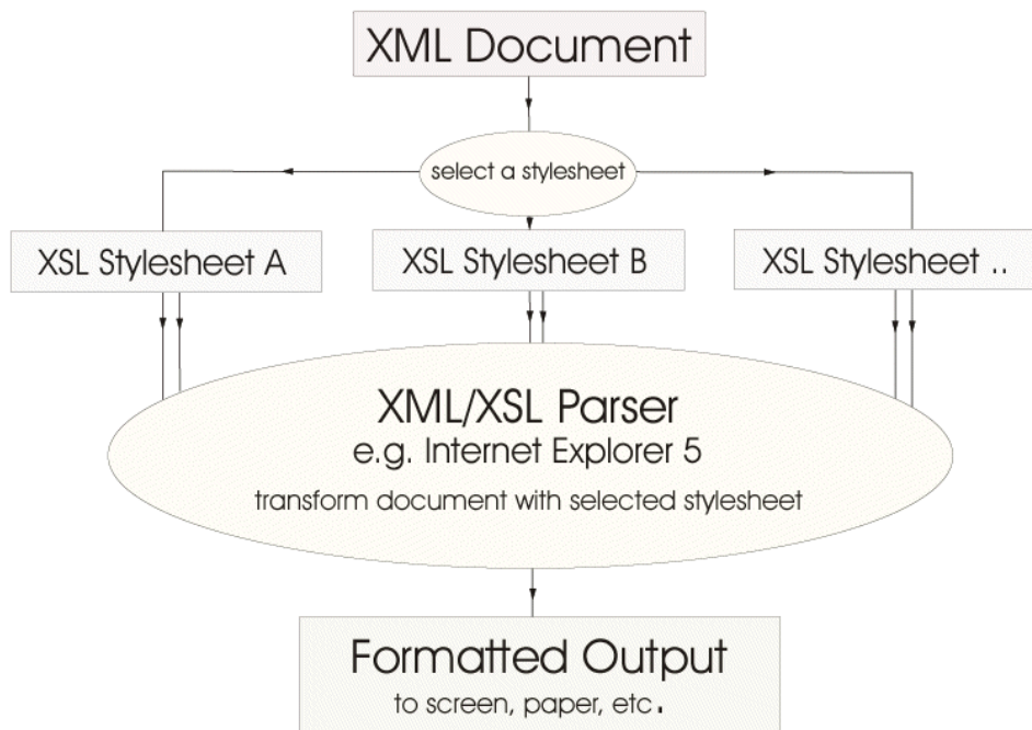
Figure 1: Data flow in an XML/XSL transform - an XML document can be transformed by one of many stylesheets depending on the required output.
