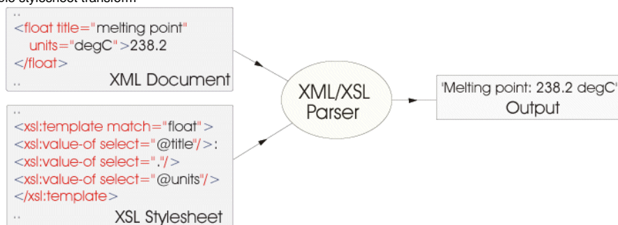
Figure 5: Simple stylesheet transform
