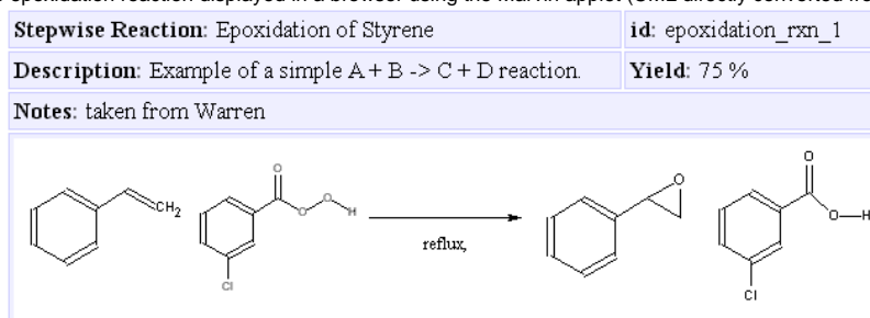
Figure 19: Stepwise epoxidation reaction displayed in a browser using the Marvin applet (CML directly converted from a rxn file)
