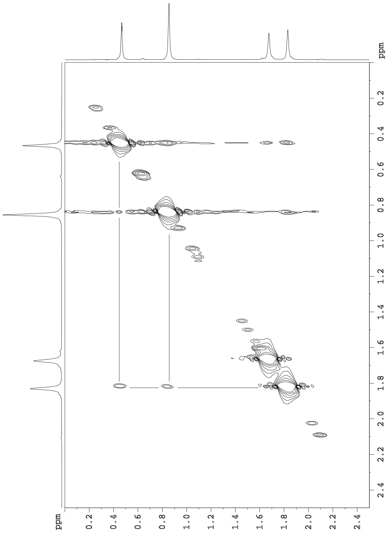
NOESY ^1\text{H} - ^1\text{H} correlation spectrum of 1
