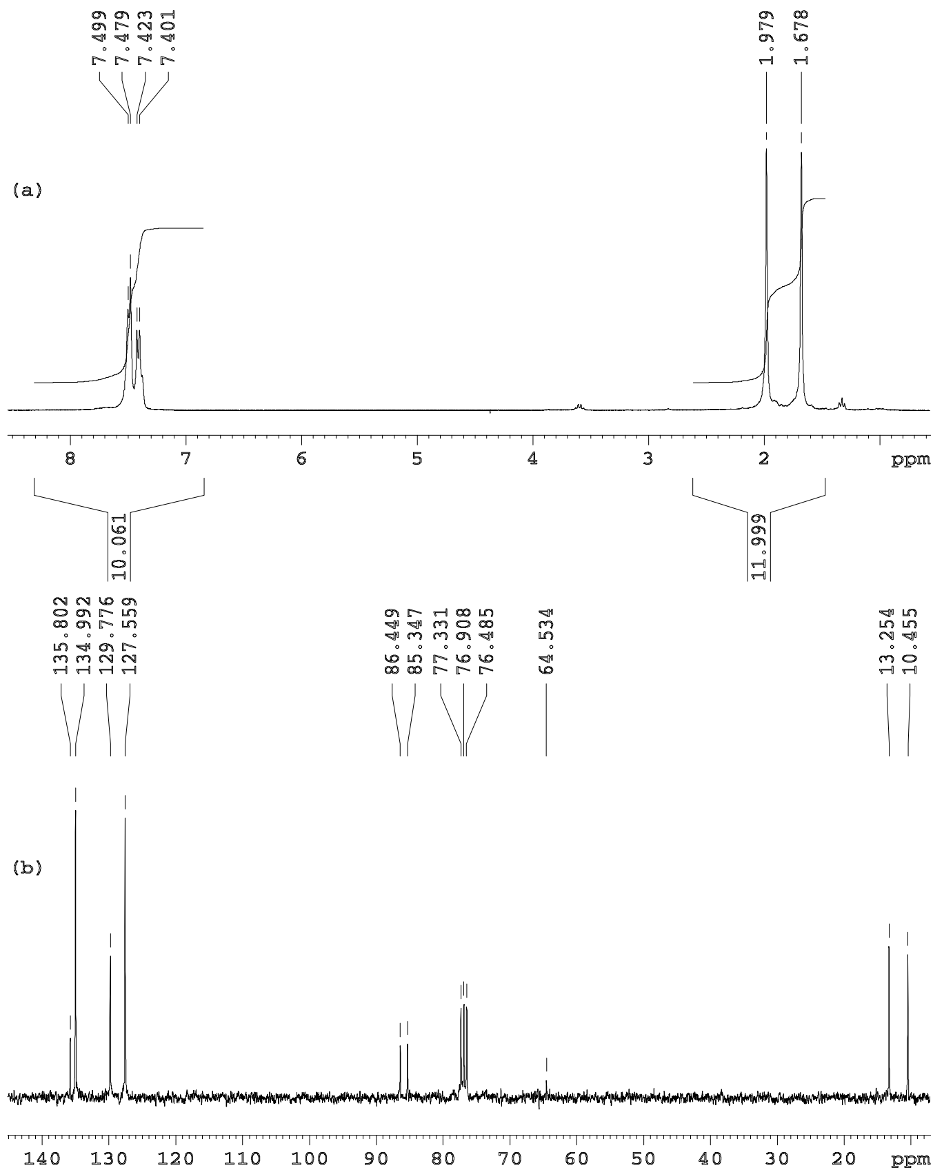
(a) ^1\text{H} and (b) ^{13}\text{C}\{^1\text{H}\} NMR spectra of 2 ( \text{CDCl}_3 , 298 K, 7.046 T)
