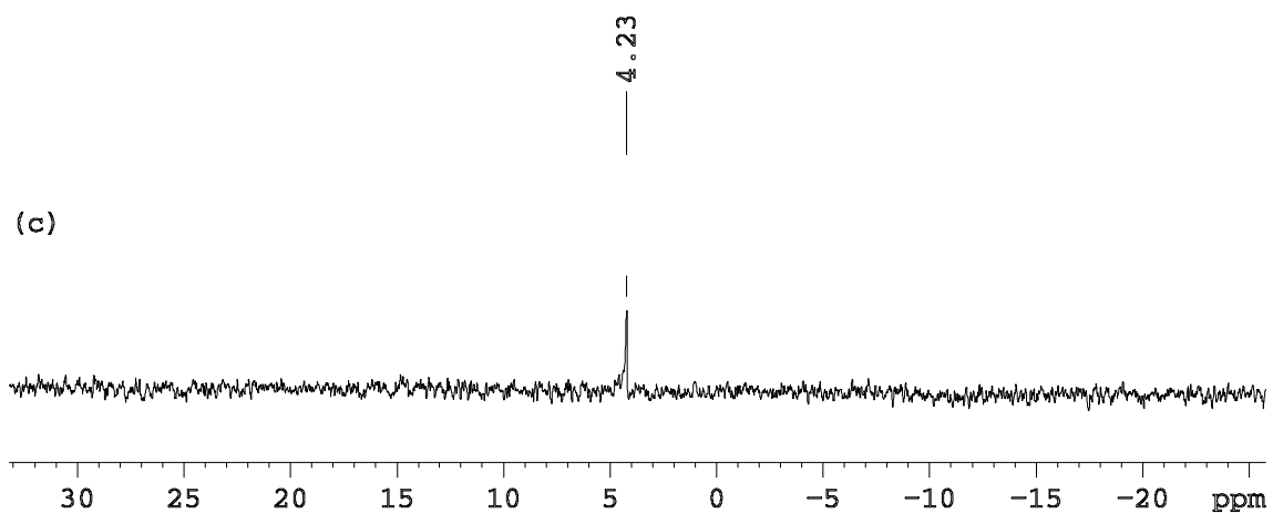
Expanded ^1\text{H} , (b) expanded ^{13}\text{C}\{^1\text{H}\} ( \text{C}_6\text{D}_6 ) and (c) ^{29}\text{Si}\{^1\text{H}\} ( \text{C}_7\text{D}_8 ) NMR spectra of 1 (298 K, 9.395 T)
